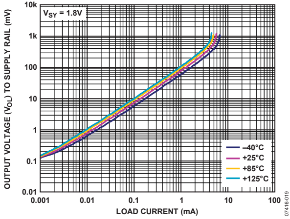
Figure 16. Output Voltage ( V_{O_i} ) to Supply Rail vs. Load Current and Temperature
