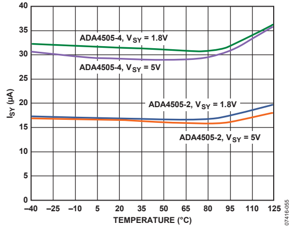
Figure 43. Total Supply Current vs. Temperature
