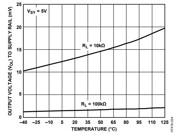
Figure 21. Output Voltage ( V_{O_i} ) to Supply Rail vs. Temperature
