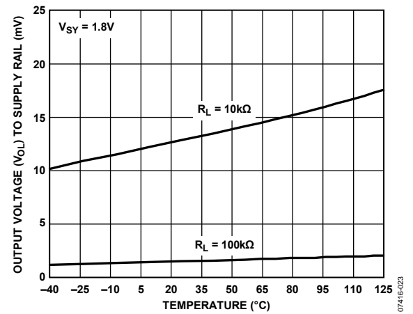
Figure 18. Output Voltage ( V_{O_i} ) to Supply Rail vs. Temperature
