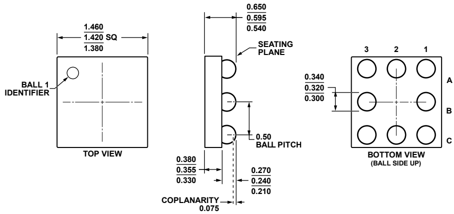
Figure 55. 8-Ball Wafer Level Chip Scale Package [WLCSP] (CB-8-2)
