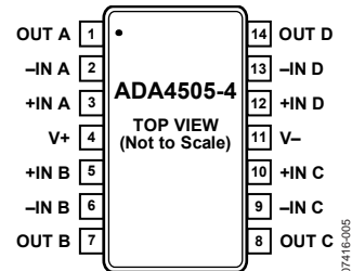
Figure 3. 14-Lead TSSOP (RU-14)
