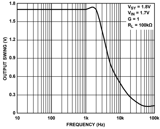
Figure 46. Output Swing vs. Frequency
